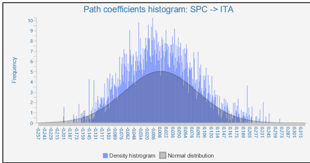
Figure 3: Normality Test.
